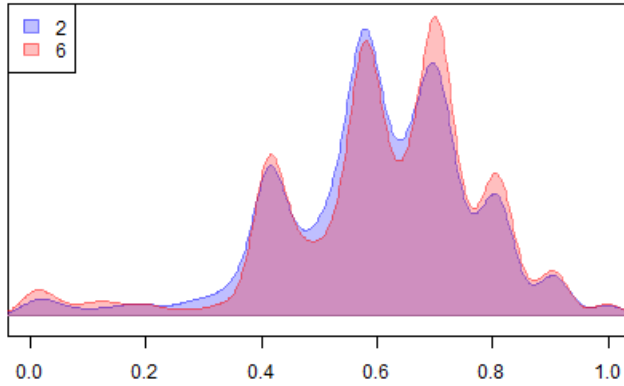
Fig. 5. The distance distributions for the 2nd and 6th set of weights calculated using the ROC method and criteria II, A, C_R . Source: author's calculations based on the FADN data
