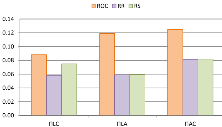
Fig. 6. Maximum values of the SM calculated for three-criteria models. Source: author's own calculations on the basis of the FADN data
